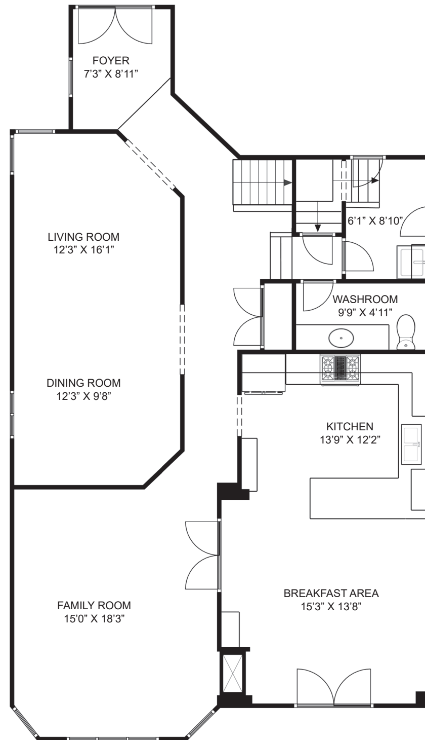
MAIN FLOOR
