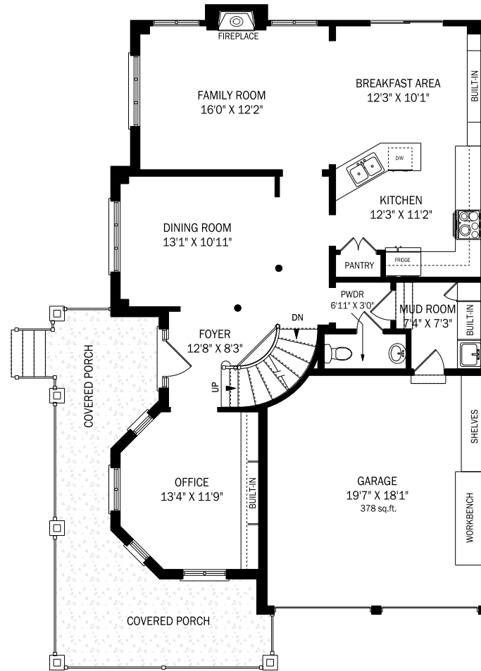
MAIN FLOOR
