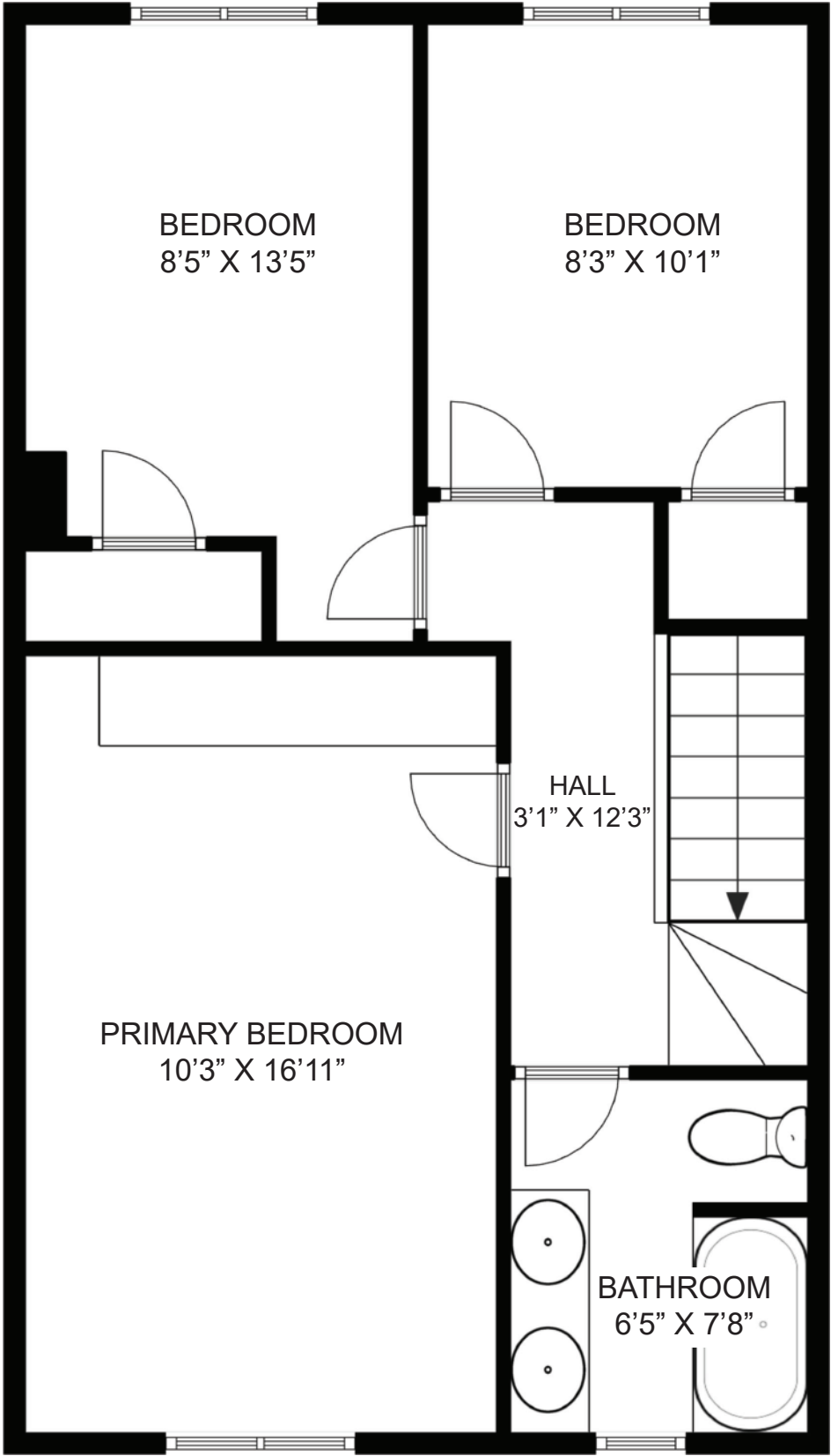
UPPER FLOOR
