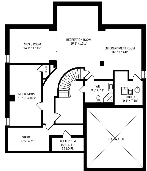
LOWER LEVEL - 1648 SQUARE FEET
