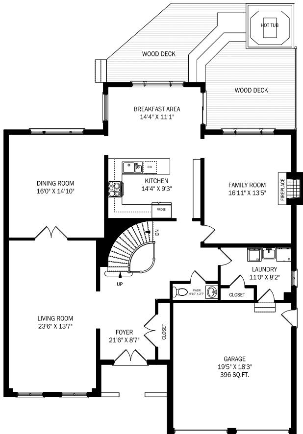
MAIN FLOOR - 1648 SQUARE FEET
