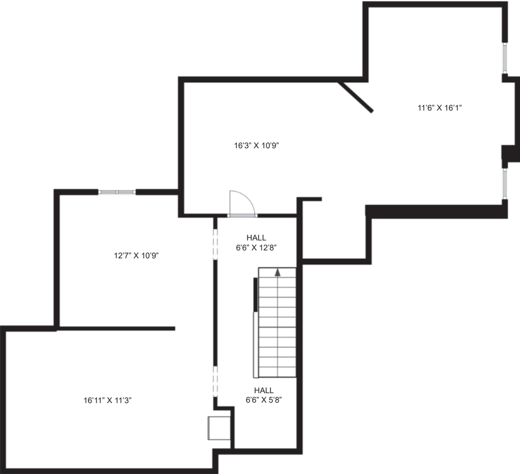
LOWER FLOOR
