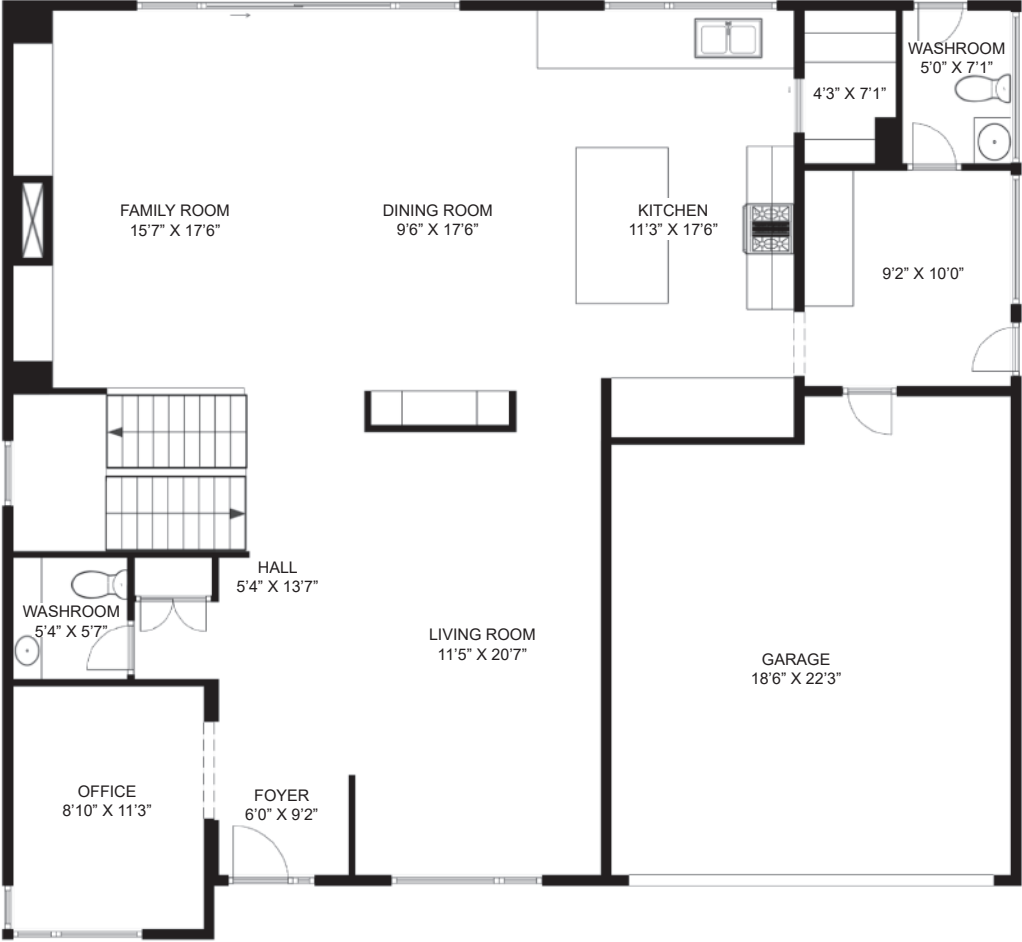
MAIN FLOOR
